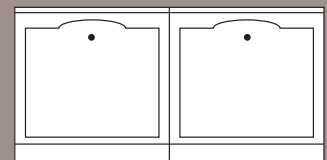
Low 2-Door Unit 3232 H:56cm (22") W:79cm (31") D:46cm (18")
